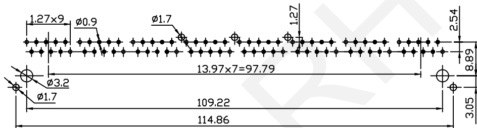
PCB Layout
